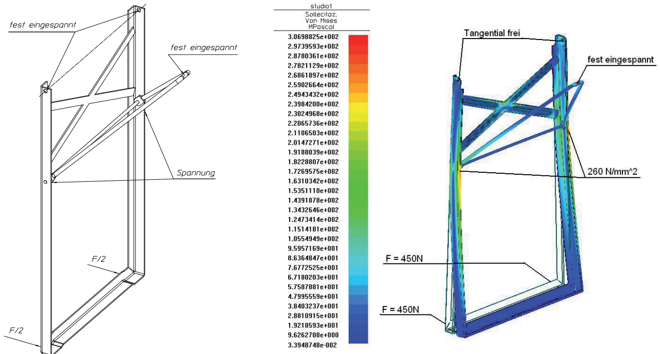
FEM table base - C-profile 25x35x8x2 tensions Material S275 (Fe430) | F= 900 N
