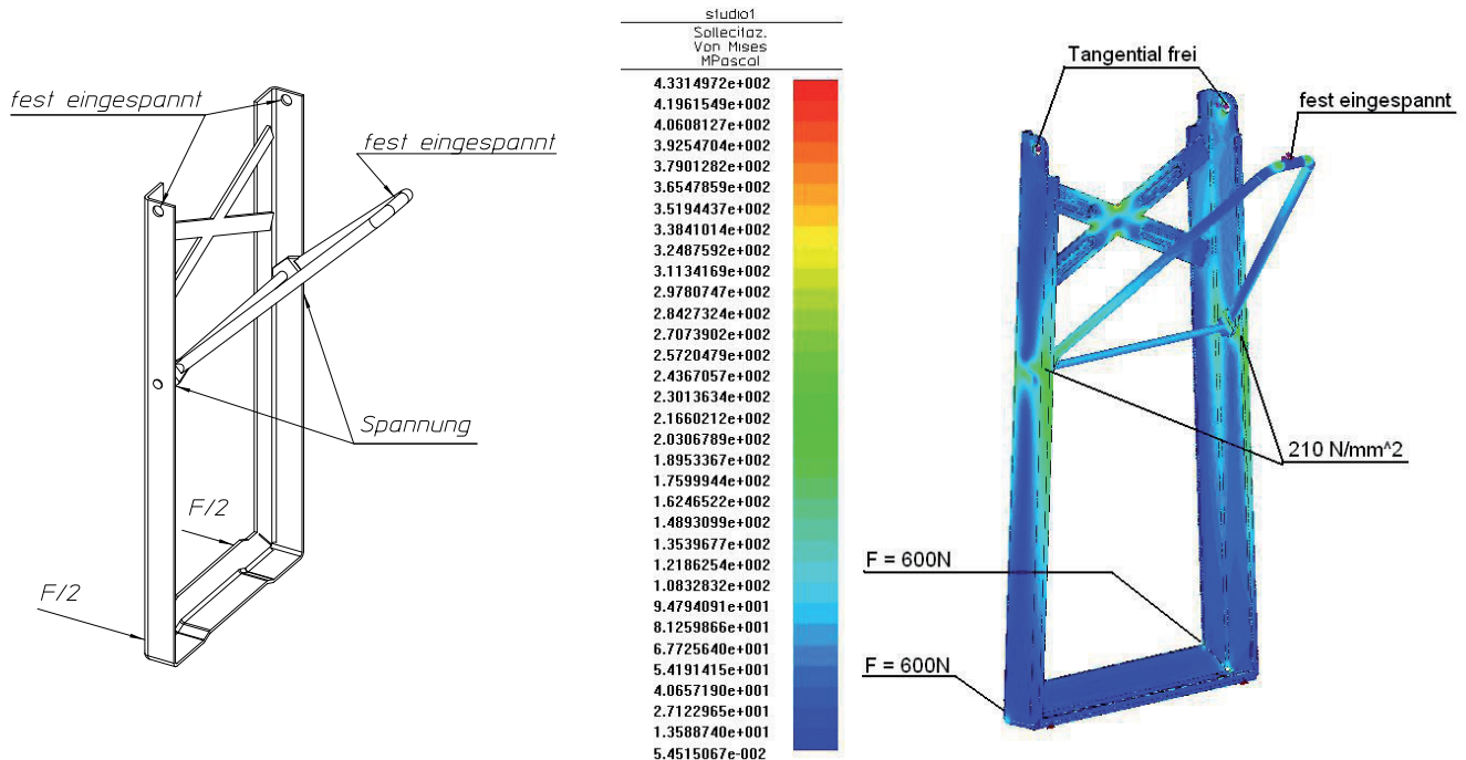
FEM bench base - C-profile 25x35x8x2 tensions Material S275 (Fe430) | F= 1200 N
